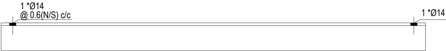
TOP VIEW
