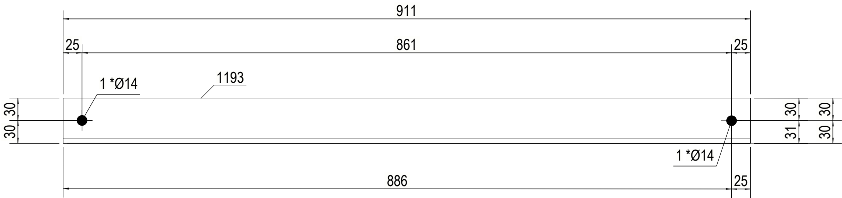
FRONT VIEW
